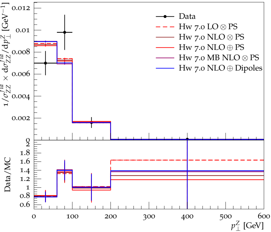
Differential cross-section for ZZ \rightarrow 4\ell vs. p_{\perp}^Z
