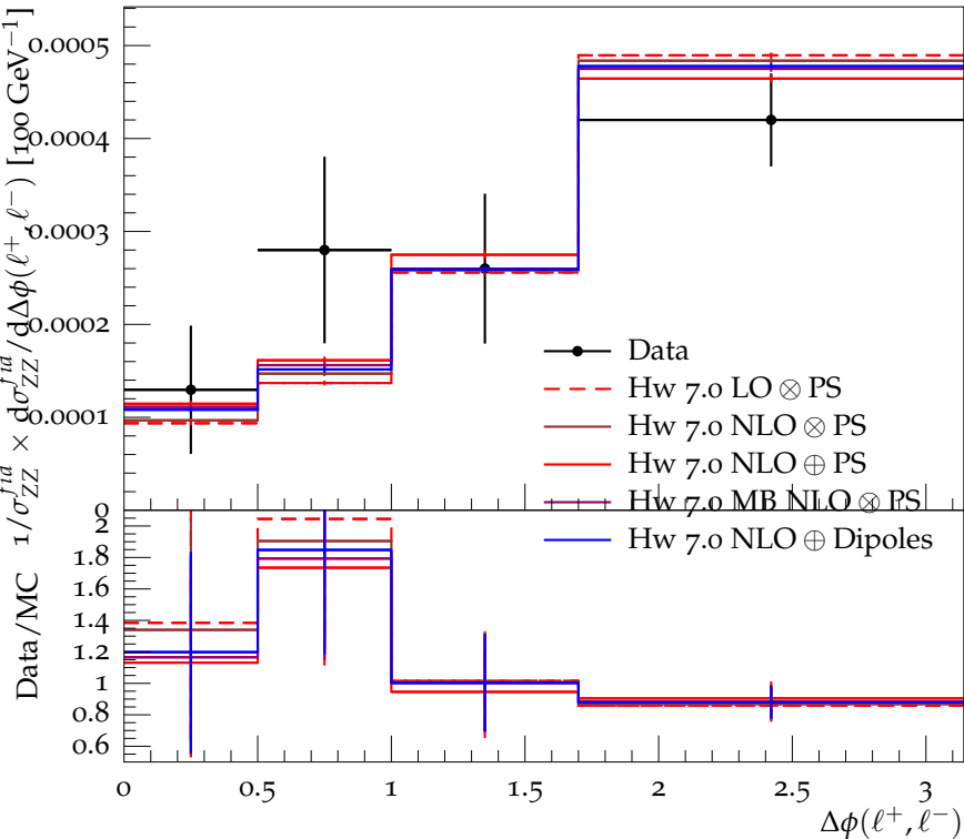
Differential cross-section for ZZ \rightarrow 4\ell vs. \Delta\phi(\ell^+, \ell^-)
