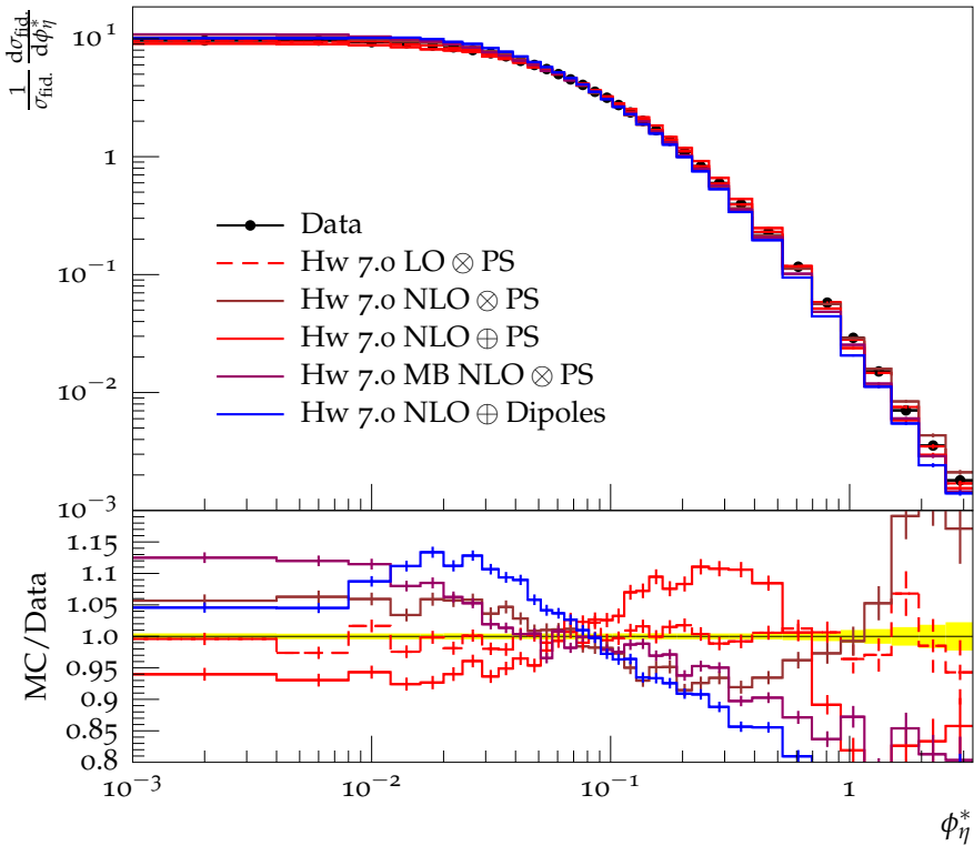
\phi_\eta^* spectrum, Z \rightarrow \mu\mu (bare)
