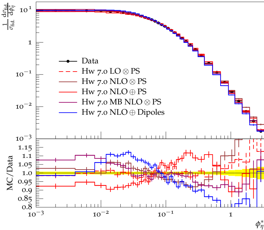
\phi_\eta^* spectrum, Z \rightarrow ee (bare), |y_Z| < 0.8
