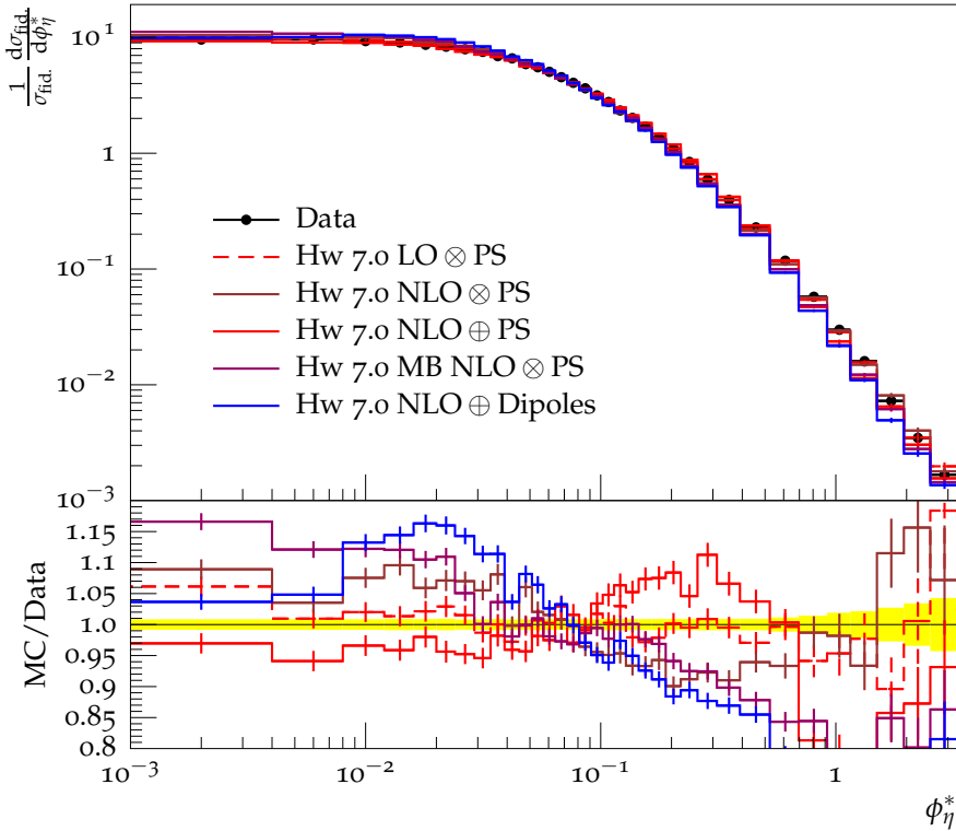
\phi_\eta^* spectrum, Z \rightarrow ee (dressed), 0.8 \leq |y_Z| < 1.6
