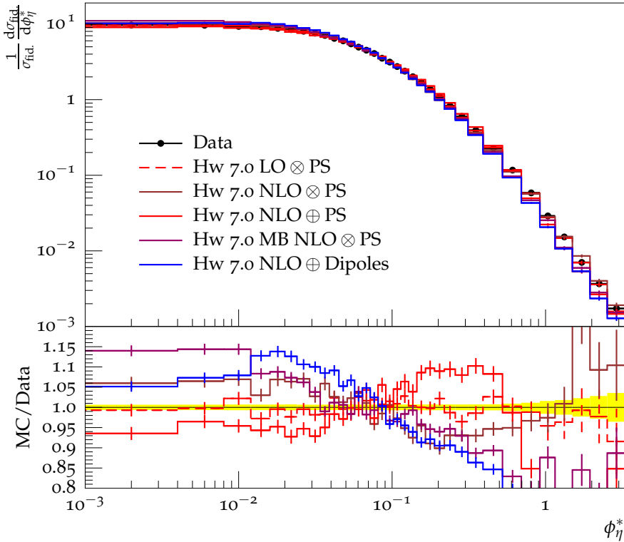
\phi_\eta^* spectrum, Z \rightarrow \mu\mu (bare), 0.8 \leq |y_Z| < 1.6
