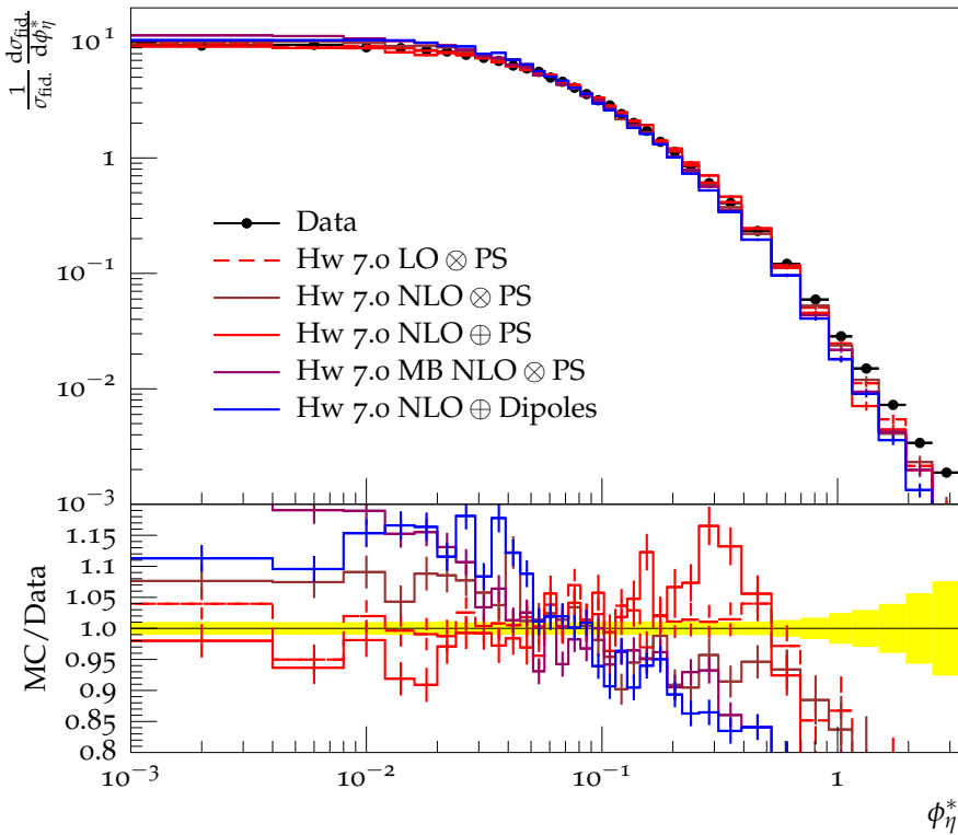
\phi_\eta^* spectrum, Z \rightarrow \mu\mu (bare), |y_Z| \geq 1.6
