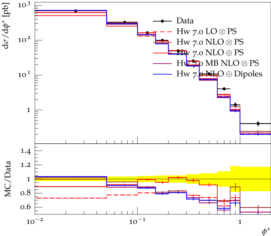
Differential cross-section for pp \rightarrow Z \rightarrow e^+e^- at \sqrt{s} = 7 TeV
