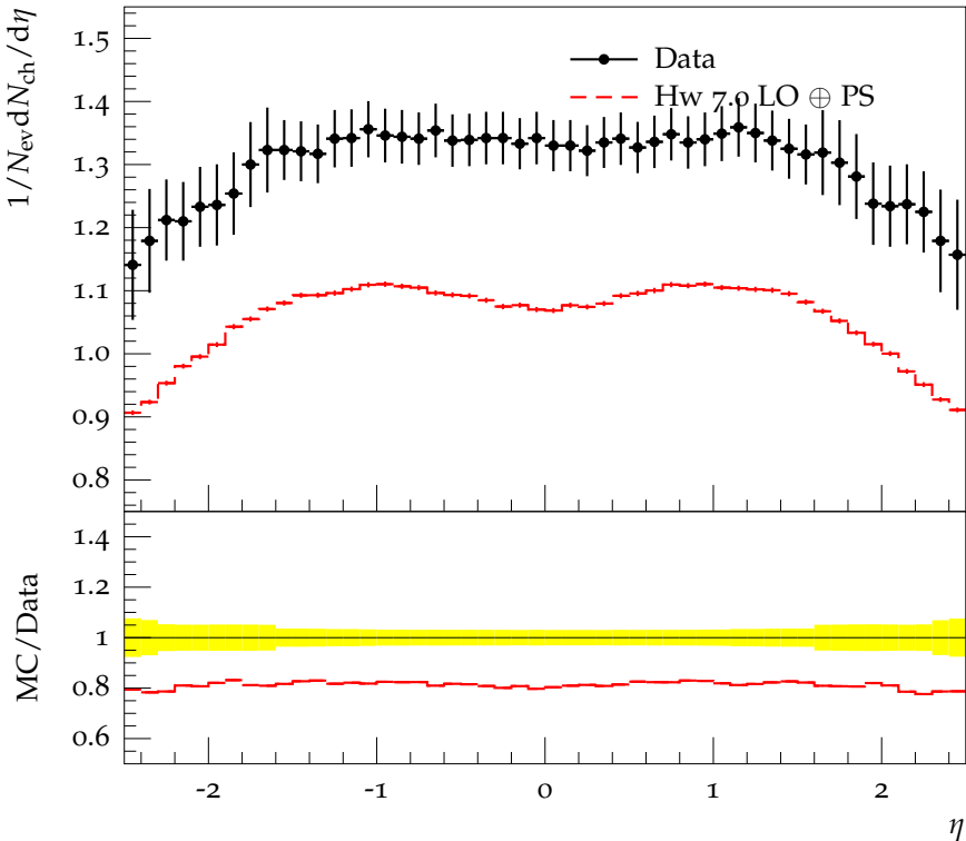
Charged particle multiplicity as function of \eta
