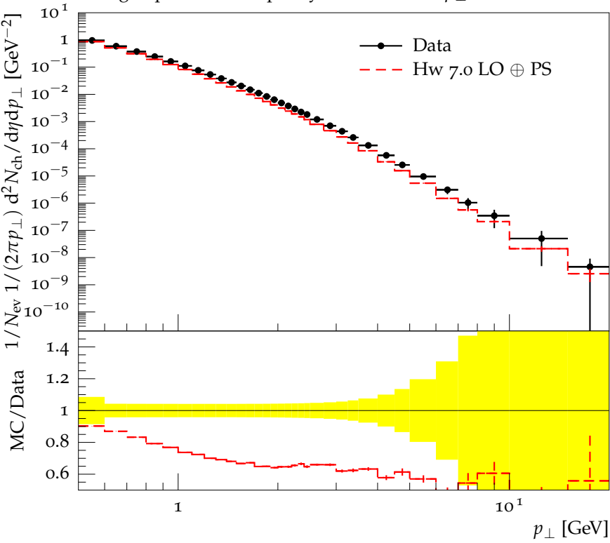
Charged particle multiplicity as function of p_{\perp}
