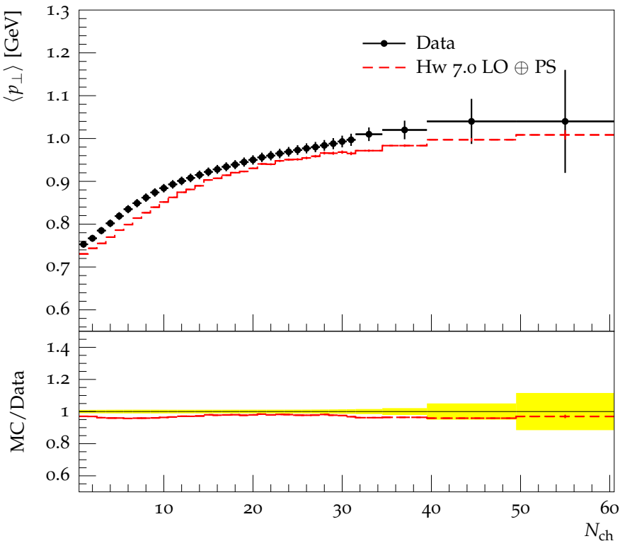
Average transverse momentum as function of N_{\text{ch}}
