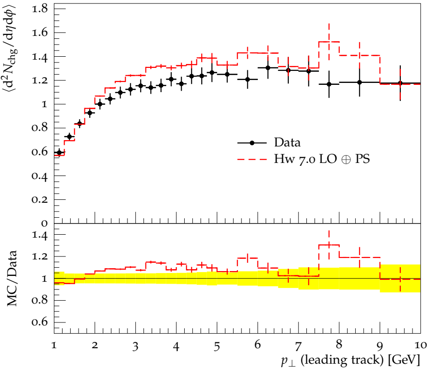
Toward N_{\text{chg}} density vs. p_{\perp}^{\text{trk1}} , \sqrt{s} = 900 GeV, p_{\perp} > 100 MeV
