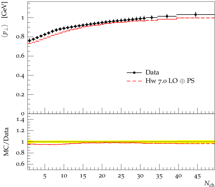
Charged \langle p_{\perp} \rangle vs. N_{\text{ch}} at 900 GeV, track p_{\perp} > 500 MeV, for N_{\text{ch}} \geq 1
