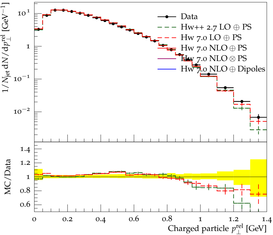
Charged jet p_{\perp}^{\text{rel}} (anti- k_t , R = 0.4 , y 0.0-1.9, p_{\perp} 10.0-15.0)
