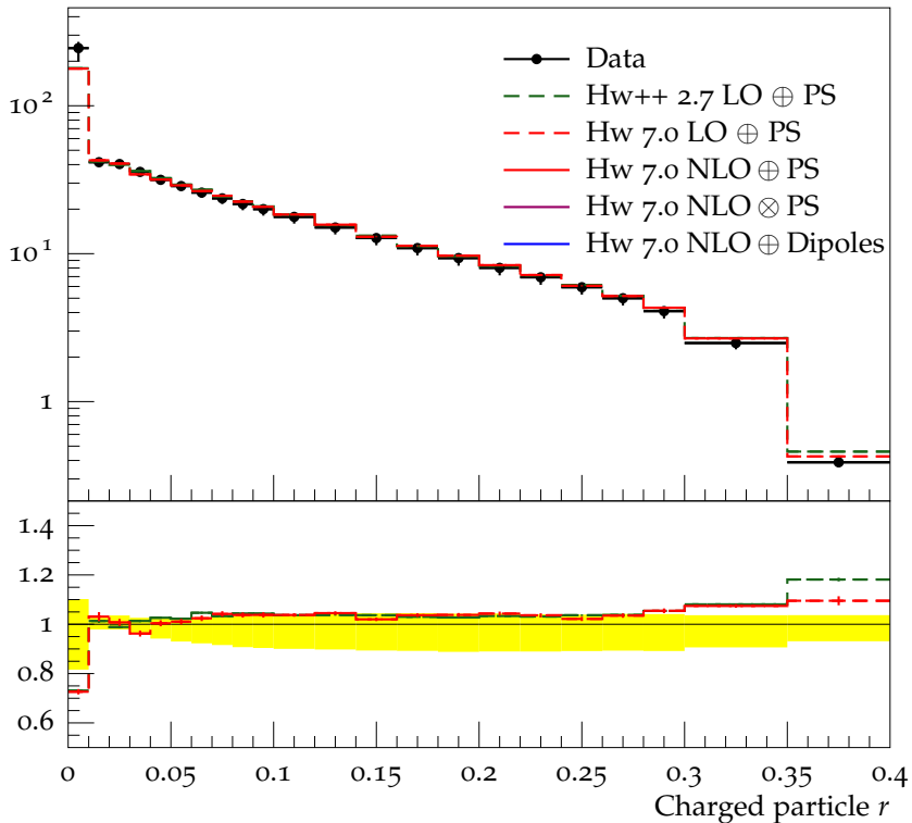
Charged jet \rho_{\text{ch}}(r) (anti- k_t , R = 0.4 , y 0.0-1.9, p_{\perp} 4.0-6.0)
