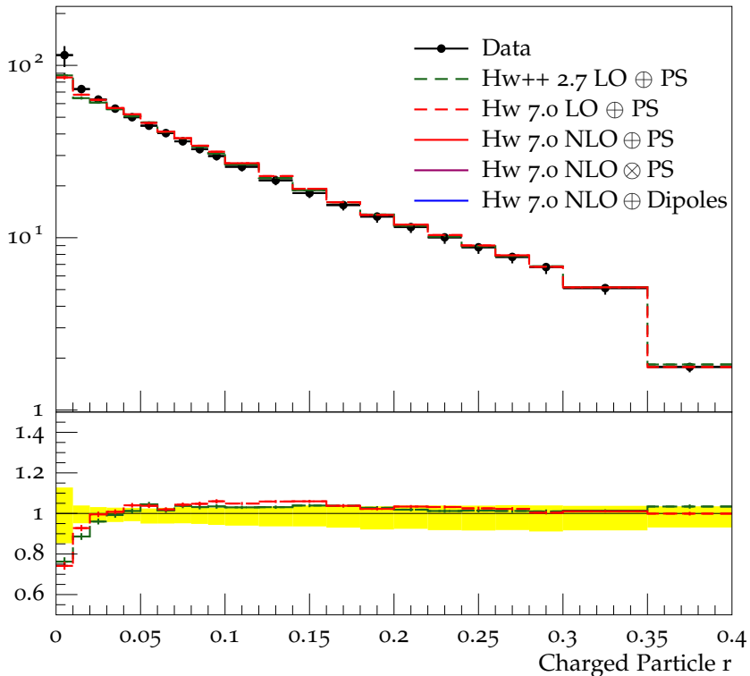
Charged jet \rho_{\text{ch}}(r) (anti- k_t , R = 0.4 , y 0.0-1.9, p_{\perp} 10.0-15.0)
