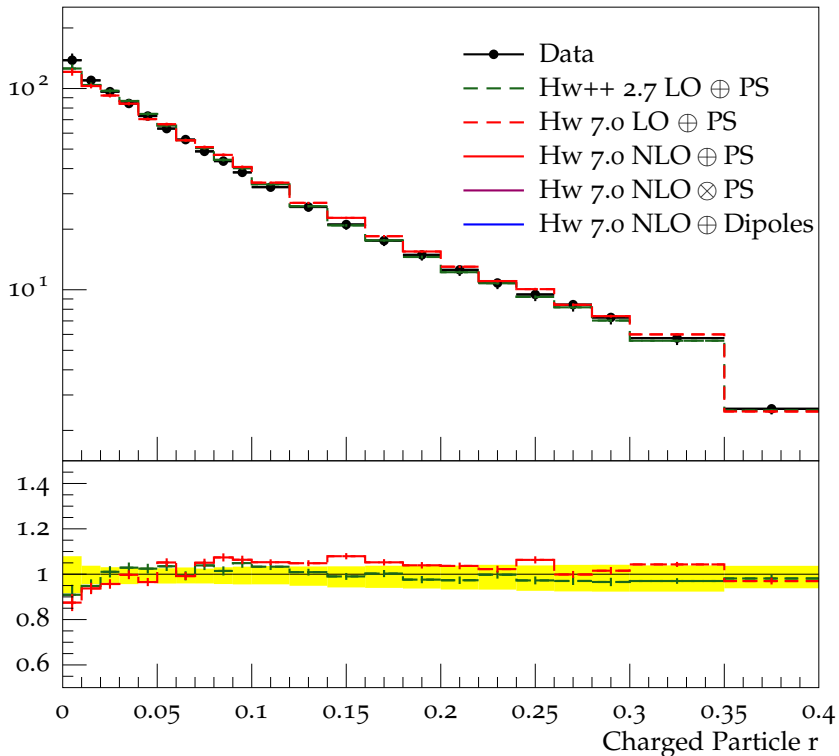
Charged jet \rho_{\text{ch}}(r) (anti- k_t , R = 0.4 , y 0.0-1.9, p_{\perp} 15.0-24.0)
