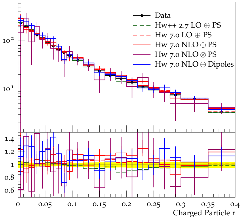
Charged jet \rho_{\text{ch}}(r) (anti- k_t , R = 0.4 , y 0.0-1.9, p_{\perp} 24.0-40.0)
