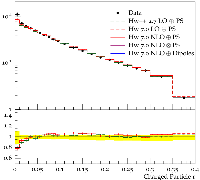
Charged jet \rho_{\text{ch}}(r) (anti- k_t , R = 0.4 , y 0.0-0.5, p_{\perp} 10.0-15.0)
