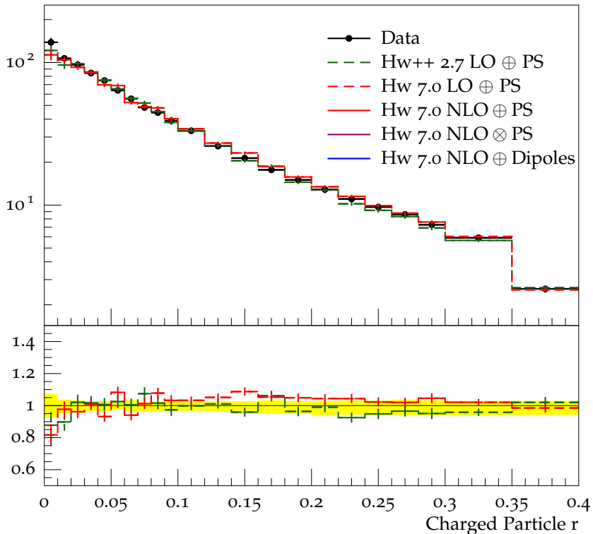
Charged jet \rho_{\text{ch}}(r) (anti- k_t , R = 0.4 , y 0.0-0.5, p_{\perp} 15.0-24.0)
