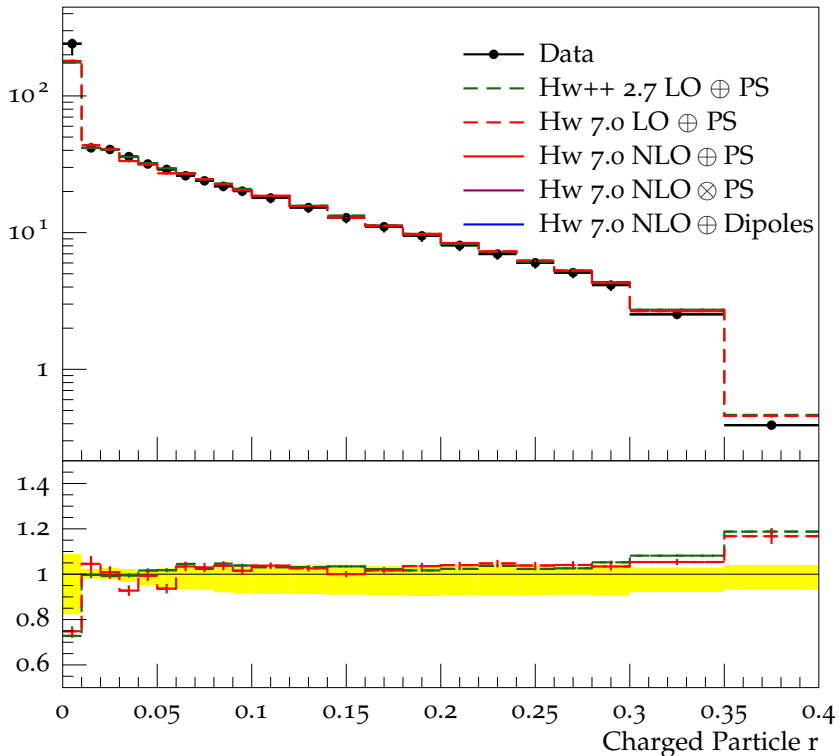
Charged jet \rho_{\text{ch}}(r) (anti- k_t , R = 0.4 , y 0.5-1.0, p_{\perp} 4.0-6.0)
