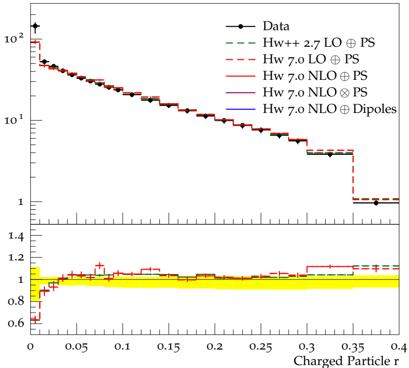
Charged jet \rho_{\text{ch}}(r) (anti- k_t , R = 0.4 , y 0.5-1.0, p_{\perp} 6.0-10.0)
