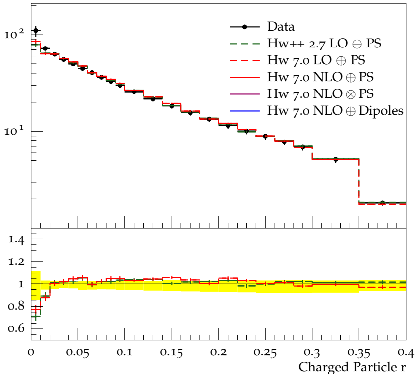
Charged jet \rho_{\text{ch}}(r) (anti- k_t , R = 0.4 , y 0.5-1.0, p_{\perp} 10.0-15.0)
