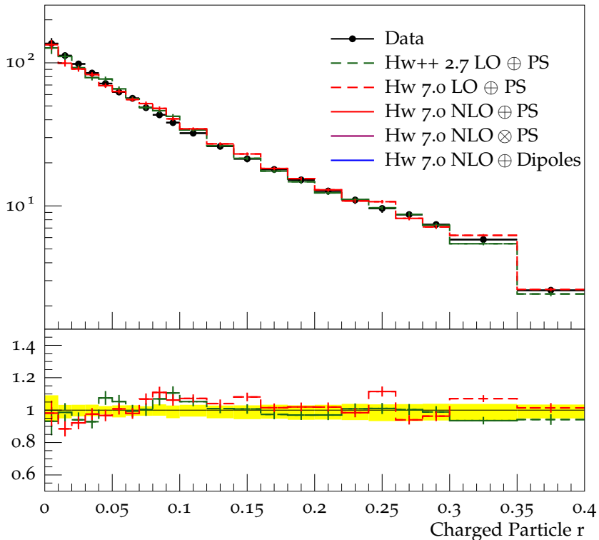
Charged jet \rho_{\text{ch}}(r) (anti- k_t , R = 0.4 , y 0.5-1.0, p_{\perp} 15.0-24.0)
