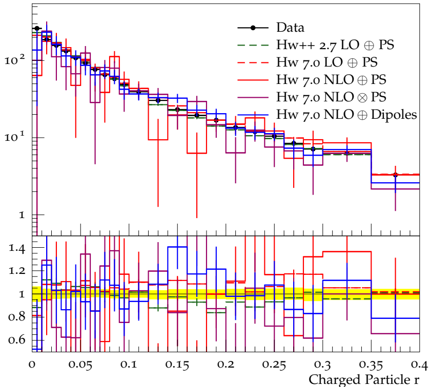
Charged jet \rho_{\text{ch}}(r) (anti- k_t , R = 0.4 , y 0.5-1.0, p_{\perp} 24.0-40.0)
