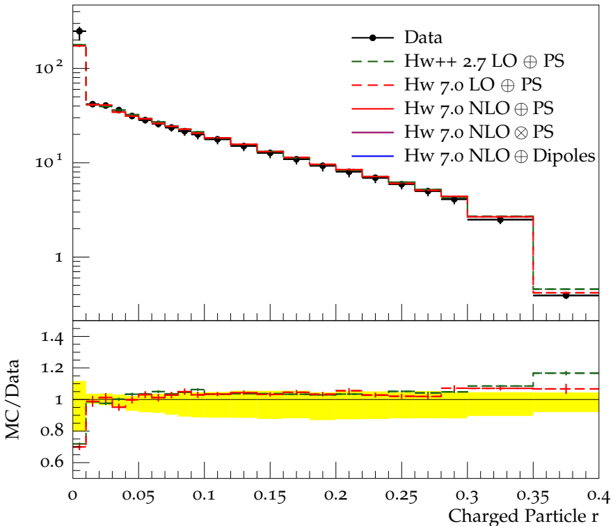
Charged jet \rho_{\text{ch}}(r) (anti- k_t , R = 0.4 , y 1.0-1.5, p_{\perp} 4.0-6.0)
