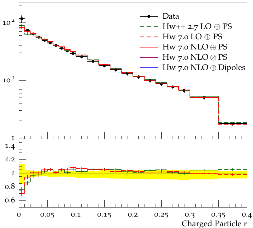
Charged jet \rho_{\text{ch}}(r) (anti- k_t , R = 0.4 , y 1.0-1.5, p_{\perp} 10.0-15.0)
