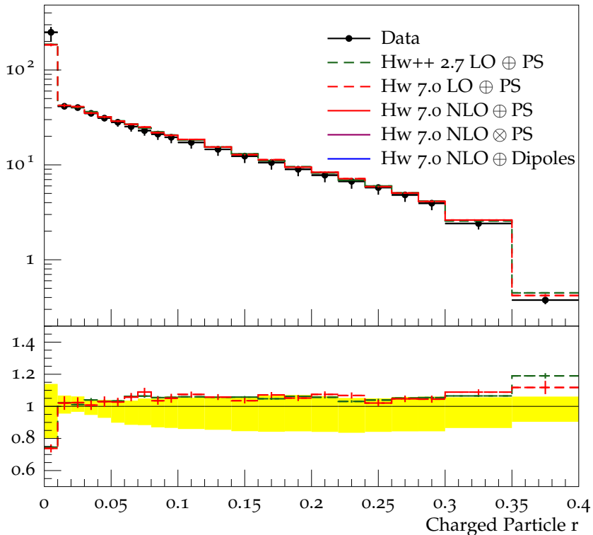
Charged jet \rho_{\text{ch}}(r) (anti- k_t , R = 0.4 , y 1.5-1.9, p_{\perp} 4.0-6.0)
