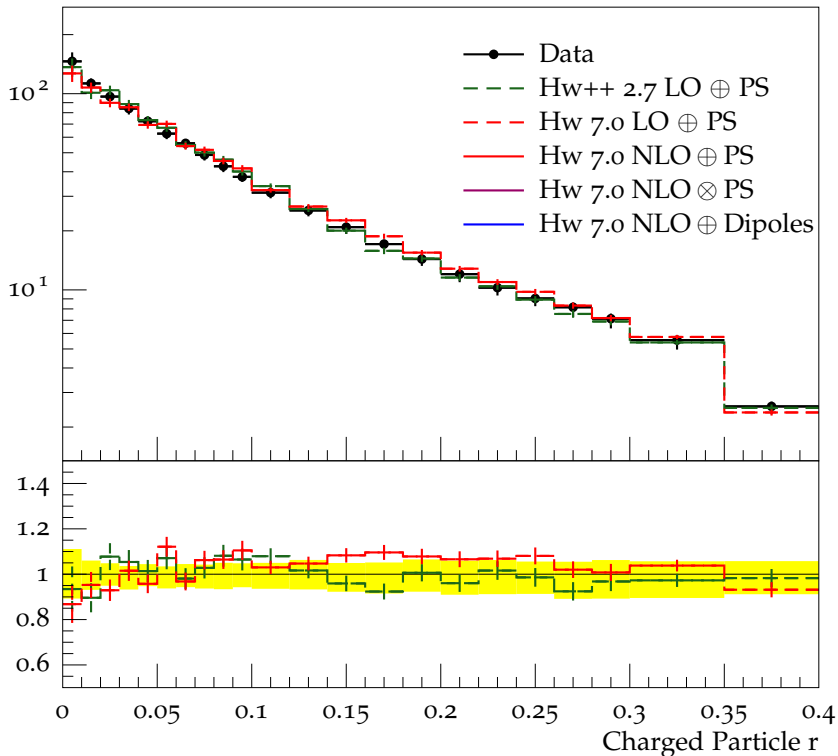
Charged jet \rho_{\text{ch}}(r) (anti- k_t , R = 0.4 , y 1.5-1.9, p_{\perp} 15.0-24.0)
