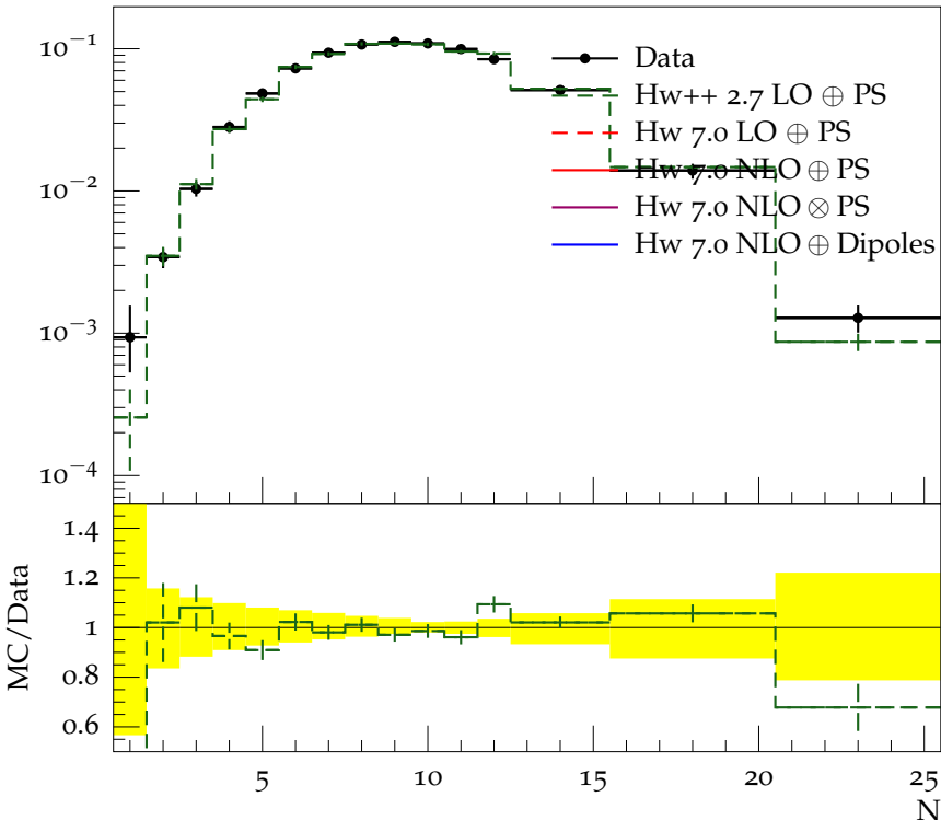
Charged jet multiplicity (anti- k_t , R = 0.6 , y 0.0-1.9, p_{\perp} 24.0-40.0)
