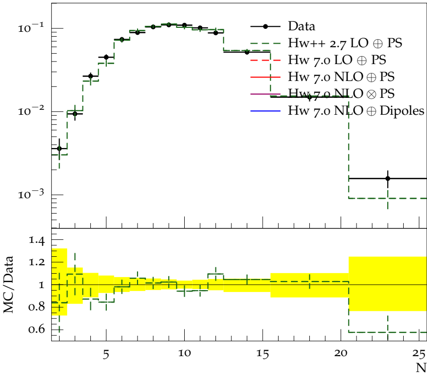
Charged jet multiplicity (anti- k_t , R = 0.6 , y 0.0-0.5, p_\perp 24.0-40.0)
