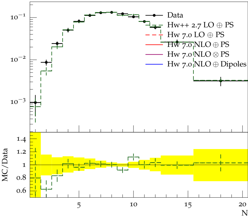
Charged jet multiplicity (anti- k_t , R = 0.6 , y 1.5-1.9, p_\perp 15.0-24.0)
