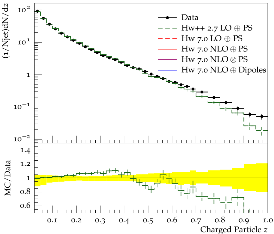
Charged jet z (anti- k_t , R = 0.6 , y 0.0-1.9, p_\perp 24.0-40.0)
