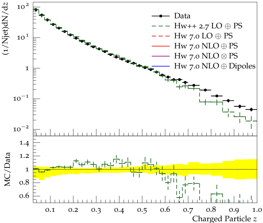
Charged jet z (anti- k_t , R = 0.6 , y 0.5-1.0, p_\perp 15.0-24.0)
