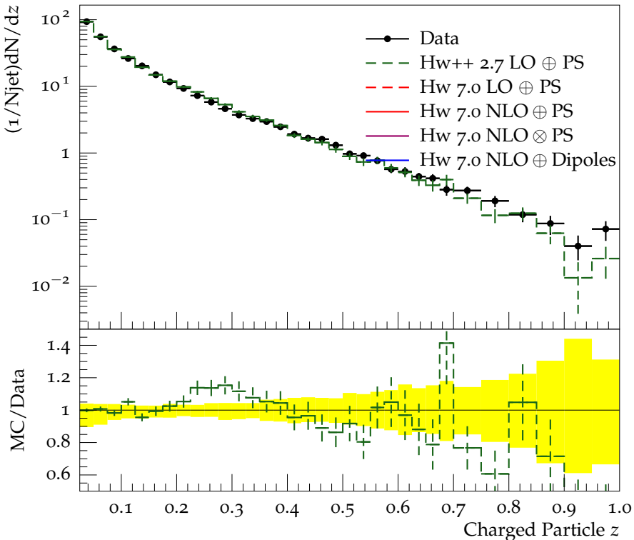
Charged jet z (anti- k_t , R = 0.6 , y 0.5-1.0, p_\perp 24.0-40.0)
