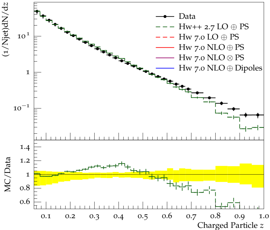
Charged jet z (anti- k_t , R = 0.6 , y 1.0-1.5, p_\perp 10.0-15.0)
