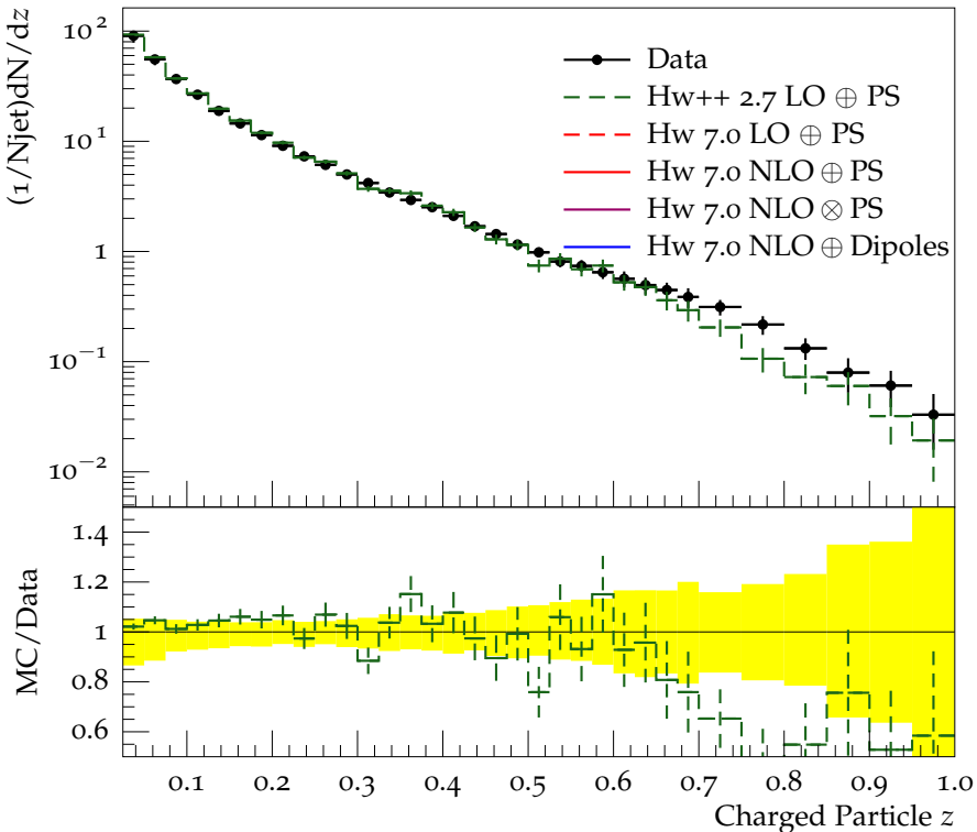
Charged jet z (anti- k_t , R = 0.6 , y 1.0-1.5, p_\perp 24.0-40.0)
