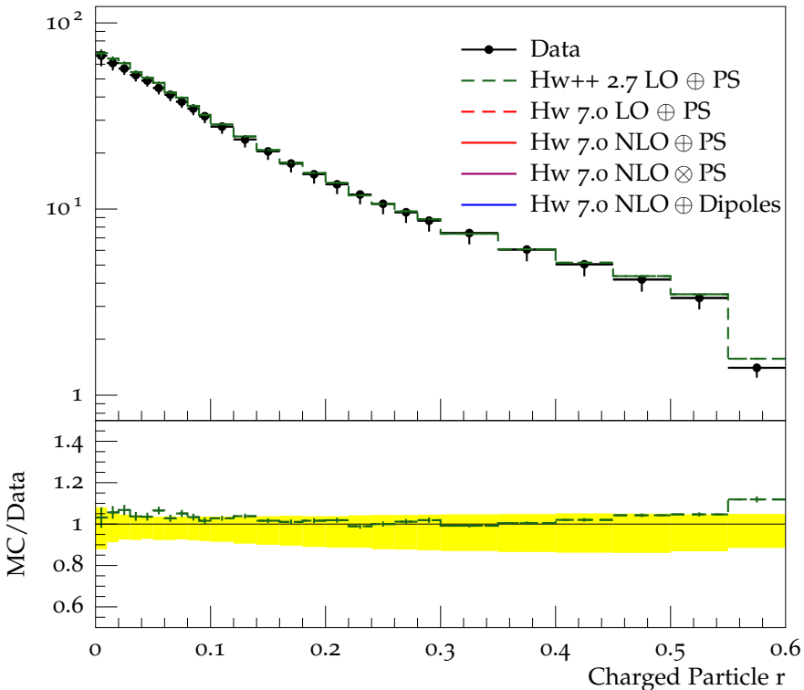
Charged jet \rho_{\text{ch}}(r) (anti- k_t , R = 0.6 , y 0.0-1.9, p_{\perp} 15.0-24.0)
