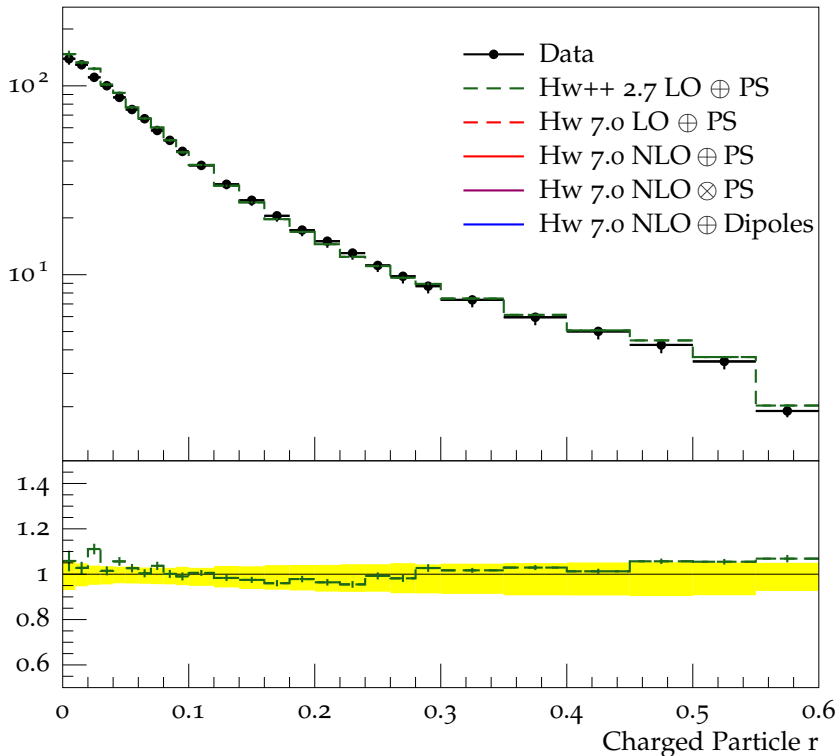
Charged jet \rho_{\text{ch}}(r) (anti- k_t , R = 0.6 , y 0.0-1.9, p_{\perp} 24.0-40.0)
