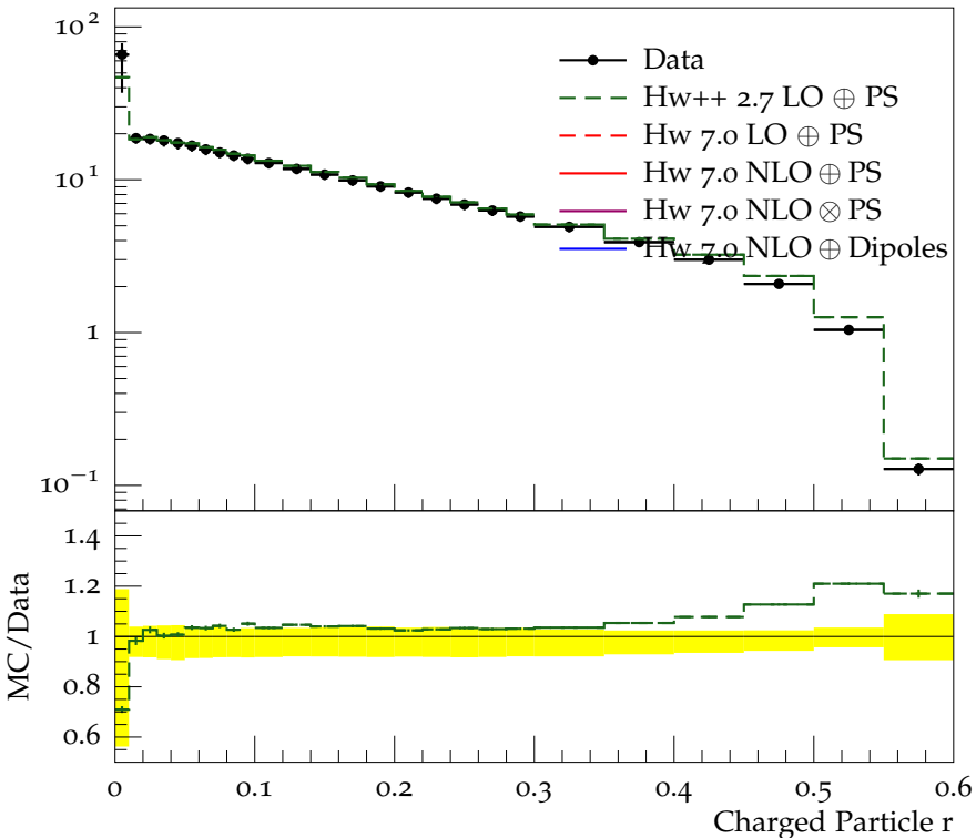
Charged jet \rho_{\text{ch}}(r) (anti- k_t , R = 0.6 , y 0.5-1.0, p_{\perp} 4.0-6.0)
