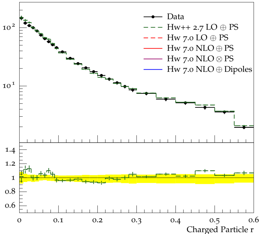
Charged jet \rho_{\text{ch}}(r) (anti- k_t , R = 0.6 , y 0.5-1.0, p_{\perp} 24.0-40.0)
