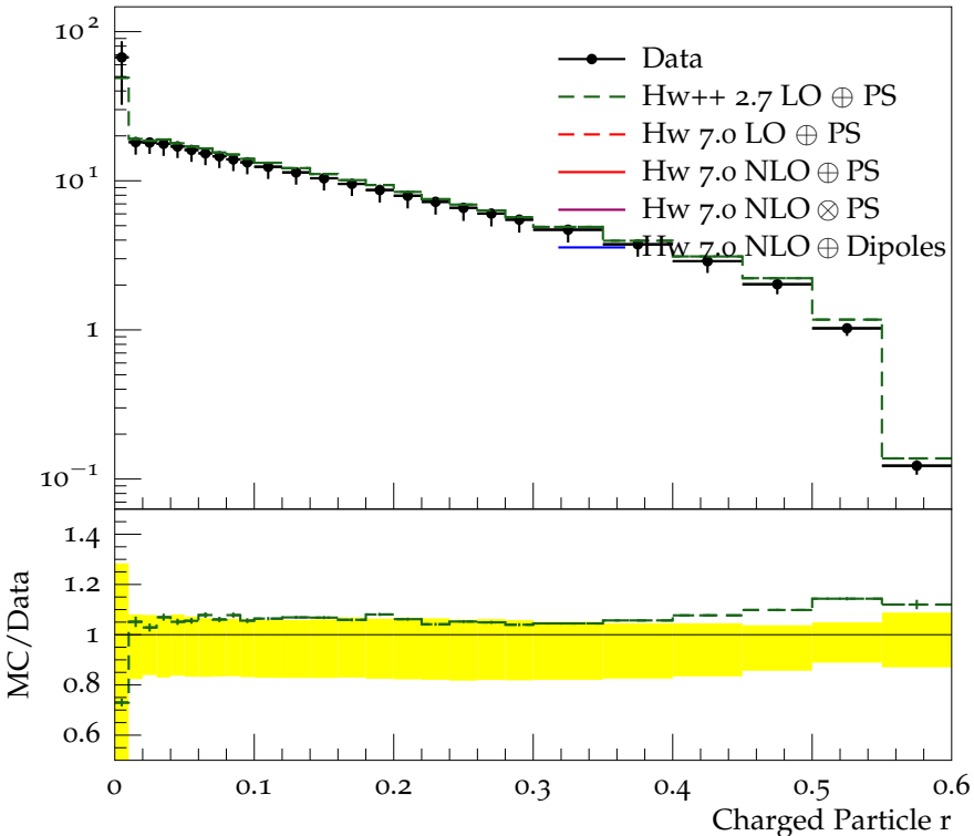
Charged jet \rho_{\text{ch}}(r) (anti- k_t , R = 0.6 , y 1.5-1.9, p_{\perp} 4.0-6.0)
