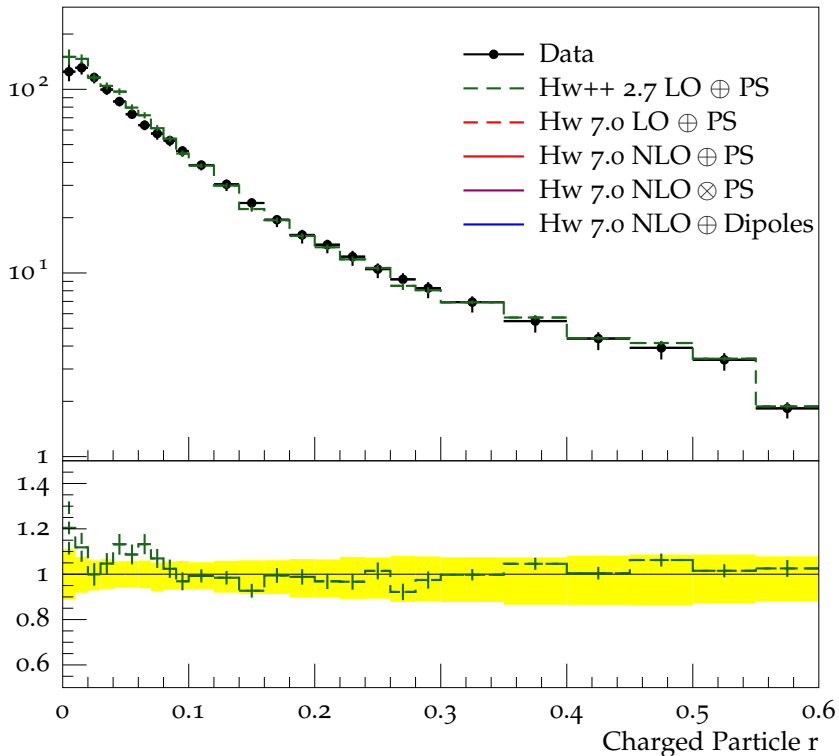
Charged jet \rho_{\text{ch}}(r) (anti- k_t , R = 0.6 , y 1.5-1.9, p_{\perp} 24.0-40.0)
