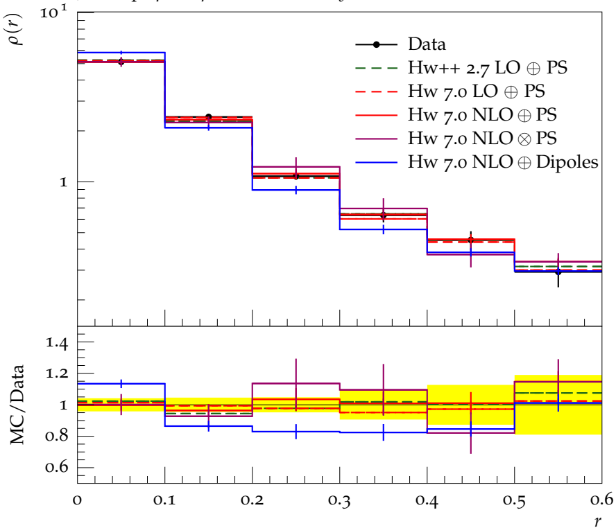
Jet shape \rho for p_{\perp} \in 60\text{--}80\text{GeV} , y \in 0.3\text{--}0.8
