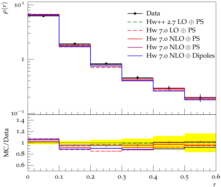
Jet shape \rho for p_{\perp} \in 110\text{--}160\text{ GeV} , y \in 0.0\text{--}2.8
