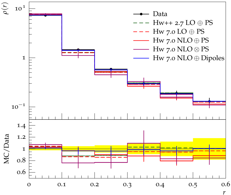
Jet shape \rho for p_{\perp} \in 160\text{--}210\text{ GeV} , y \in 2.1\text{--}2.8
