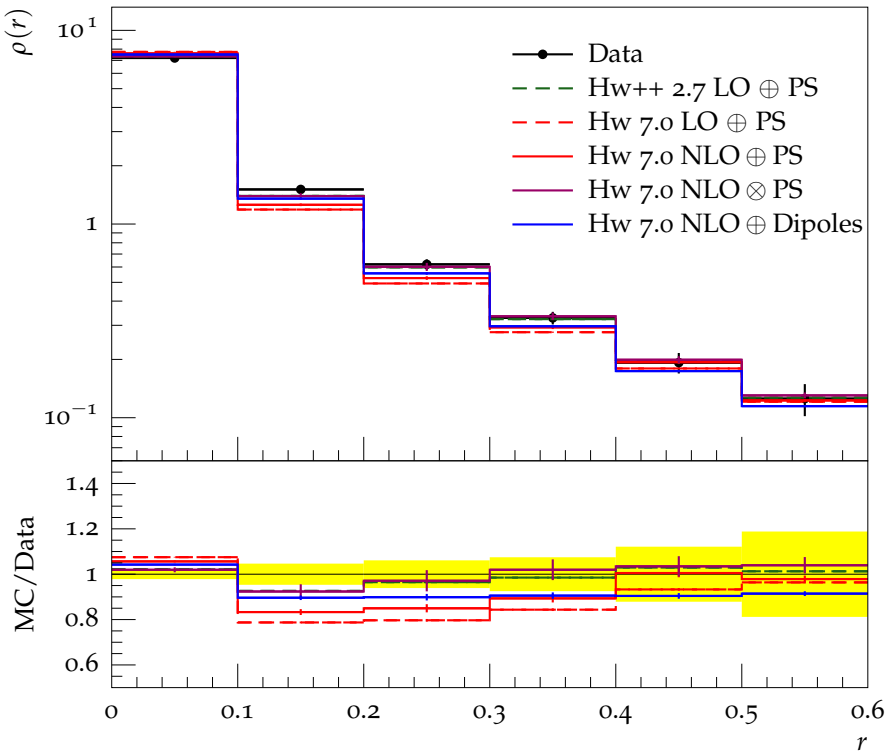
Jet shape \rho for p_{\perp} \in 210\text{--}260\text{ GeV} , y \in 1.2\text{--}2.1
