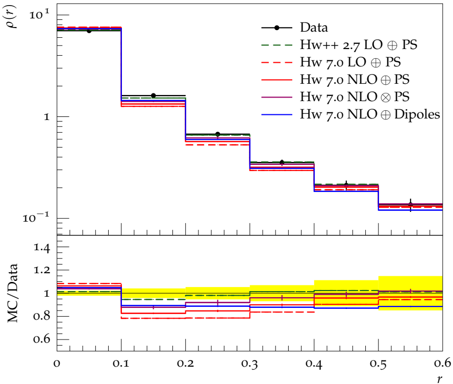
Jet shape \rho for p_{\perp} \in 210\text{--}260\text{ GeV} , y \in 0.0\text{--}2.8
