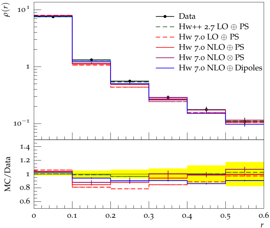
Jet shape \rho for p_{\perp} \in 260\text{--}310\text{ GeV} , y \in 1.2\text{--}2.1
