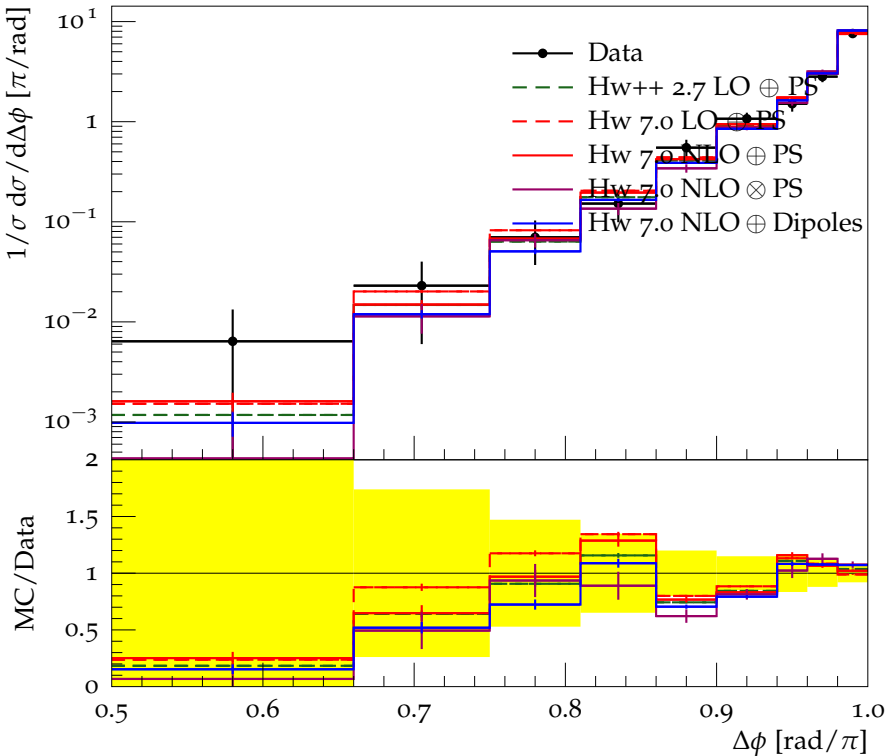
Dijet azimuthal decorrelations for 600 < p_{\perp}^{\max}/\text{GeV} < 800
